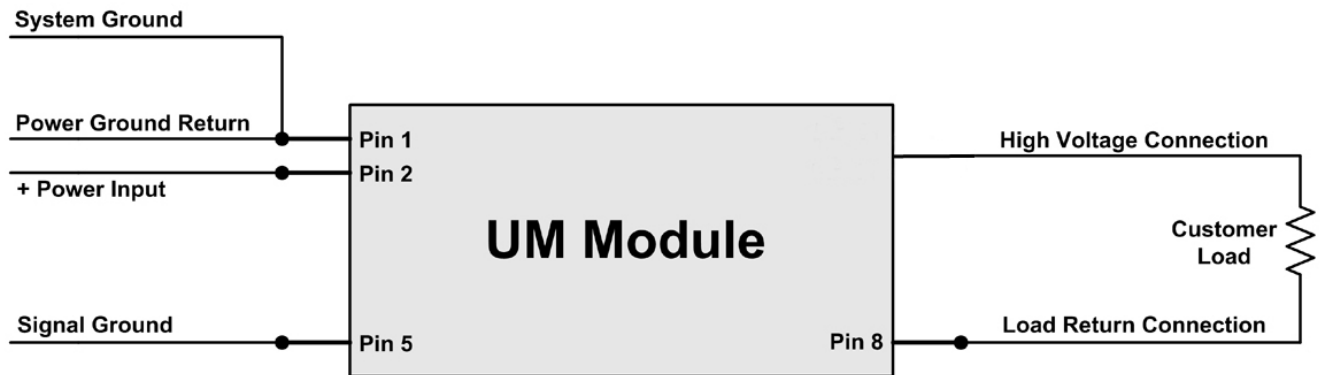
Figure 2 – Grounding
