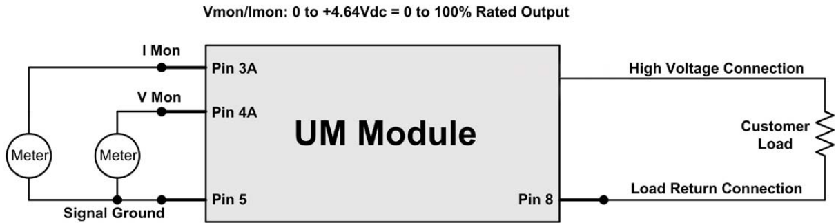
Figure 5 – Remote Voltage and Current Monitoring
