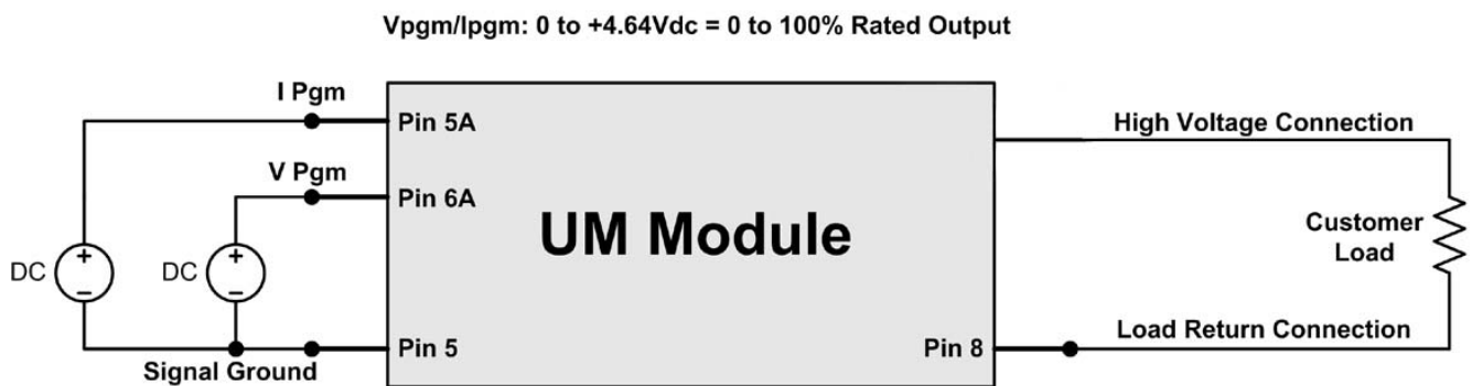
Figure 3 – Programming with a Remote Voltage Source
