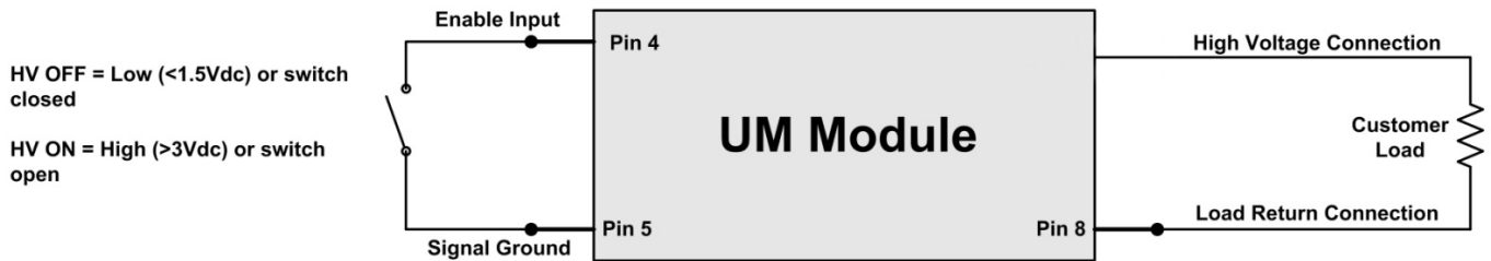
Figure 6 – Enable Input
